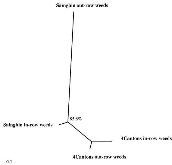
Fig. 1 Genetic relationships between in-row and out-row weeds of the two sampled fields. A Nei's genetic distance matrix between the different samples was used to draw an unrooted dendrogram by using the neighbor-joining method
