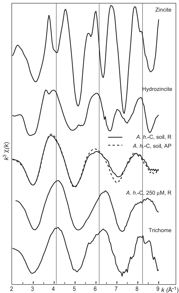
Figure 7. Comparison of the \mu EXAFS spectrum for the trichome with the powder EXAFS spectra for A.h.-C and for a selection of reference compounds.
