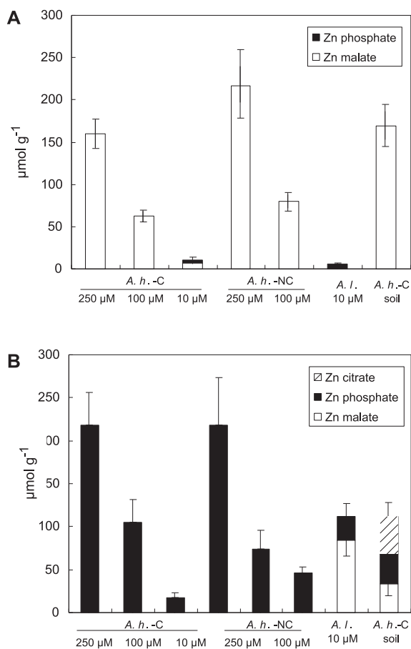
Figure 4. Concentration of Zn species in the aerial parts (A) and in the roots (B) of the plants calculated from EXAFS fitting percentages and Zn concentrations, as explained in Table II.
