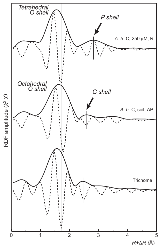
Figure 8. RDFs for the trichome and for powder samples (roots and aerial part) of A.h.-C .
