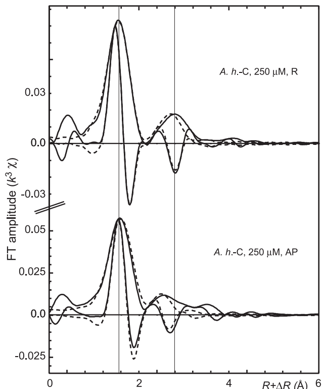
Figure 5. Radial distribution functions (RDFs; modulus and imaginary part) for the roots and the aerial parts of A.h.-C grown in solution containing 250 \mu\text{M} Zn. Solid lines are data and dashed lines are numerical simulations. EXAFS parameters are given in Table III.
