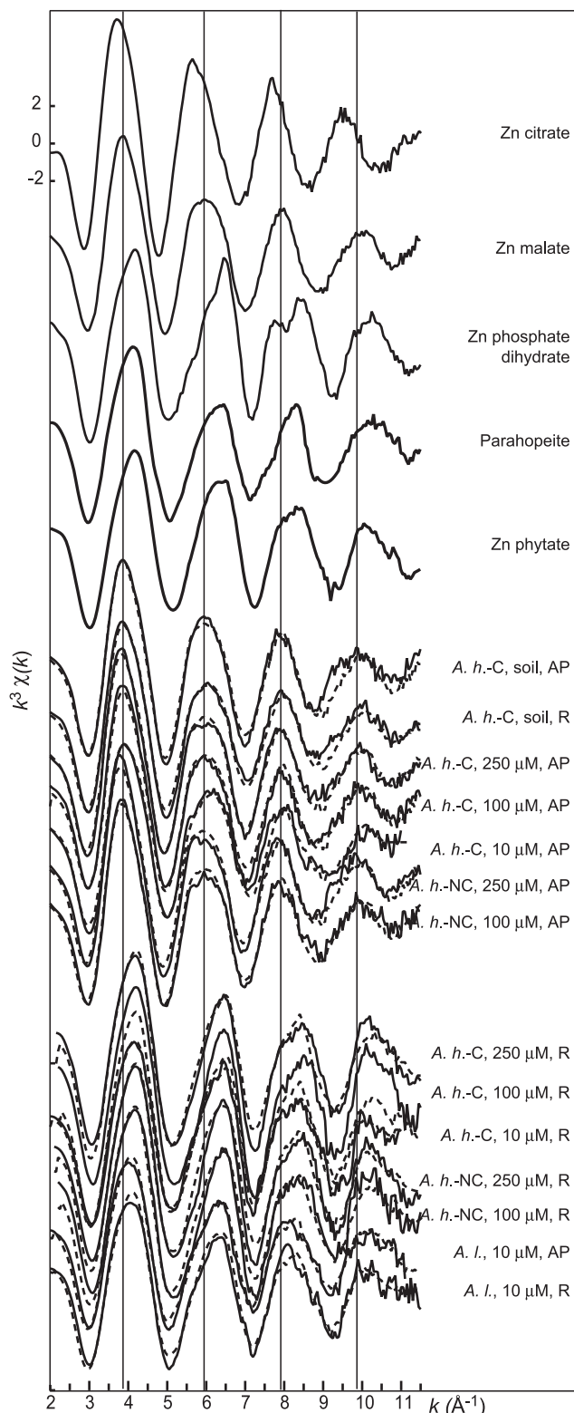
Figure 3. Zn K-edge EXAFS spectra for the plant samples ( A.h.-C ; A.h.-NC ; A.l. ; R, roots; AP, aerial parts) and for some Zn reference compounds. Solid lines are data and dashed lines are linear combinations of Zn malate and Zn phytate.
