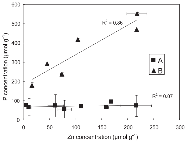
Figure 1. Relationship between Zn and P concentrations in the plant samples. Two groups of points can be defined: The first one (group A) represents the aerial parts of all plants and the roots of A. halleri from the contaminated soil. For these samples, Zn and P are not correlated ( R^2 , regression coefficient = 0.07). The second group (group B) represents the roots of all plants, except those of A. halleri from the contaminated soil. A Zn-P correlation clearly exists for these samples ( R^2 = 0.86 ).
