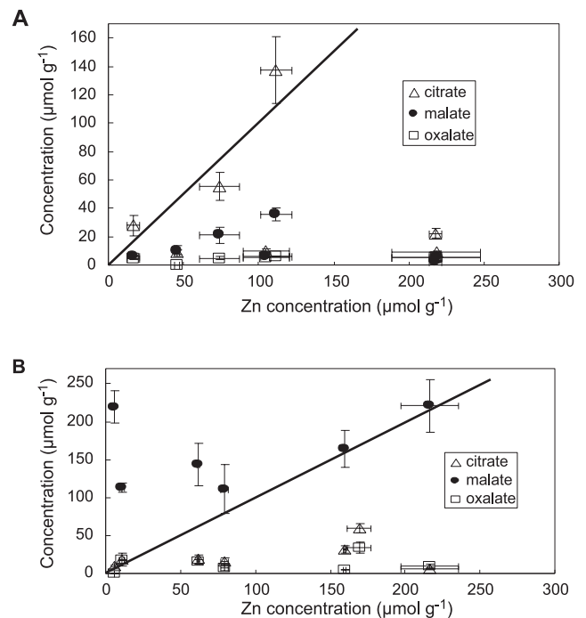
Figure 2. Organic acid content as a function of Zn content in the roots (A) and in the aerial parts (B) of the plants (values given in Table I). The line y = x is shown in each plot.
